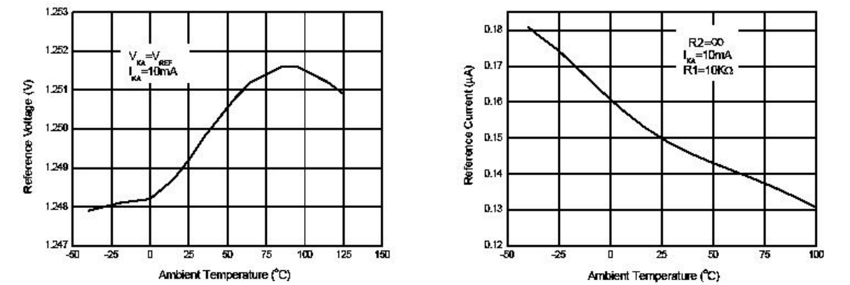
Figure 7. Reference Voltage vs. Ambient Temperature Figure 8. Reference Current vs. Ambient Temperature
