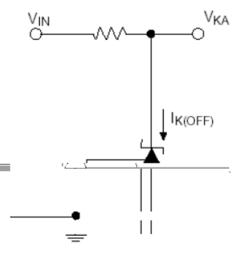
Test Circuit For I_{KA(OFF)}
