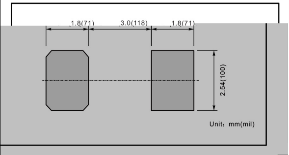
The recommended mounting pad size
