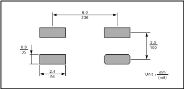
Recommended mounting pad size
