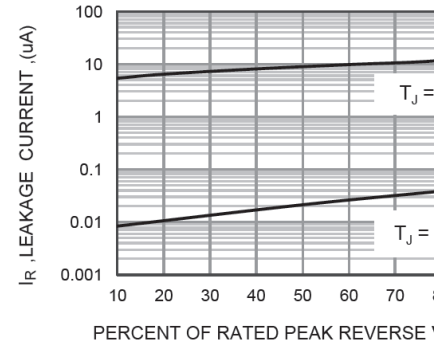
FIG.5-TYPICAL REVERSE CHARACTERISTICS
