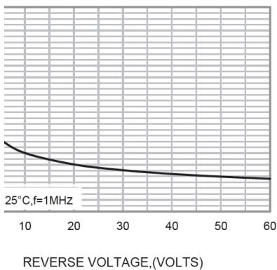
FIG.3-TYPICAL JUNCTION CAPACITANCE
