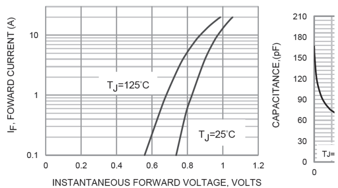
FIG.4-TYPICAL FORWARD CHARACTERISTICS
