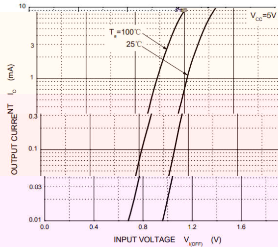
Figuer 2: OFF Characteristics
