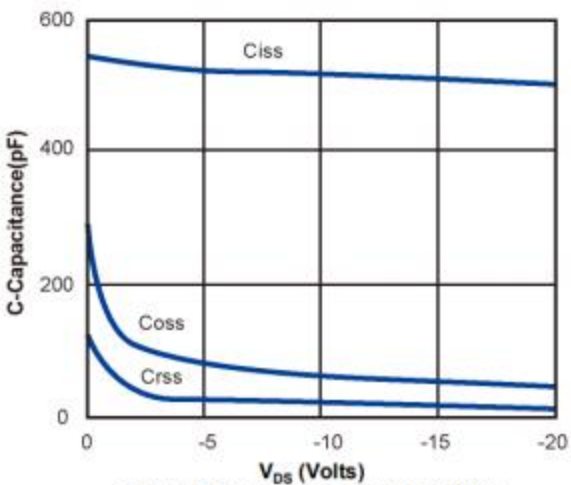
Figure 8: Capacitance Characteristics
