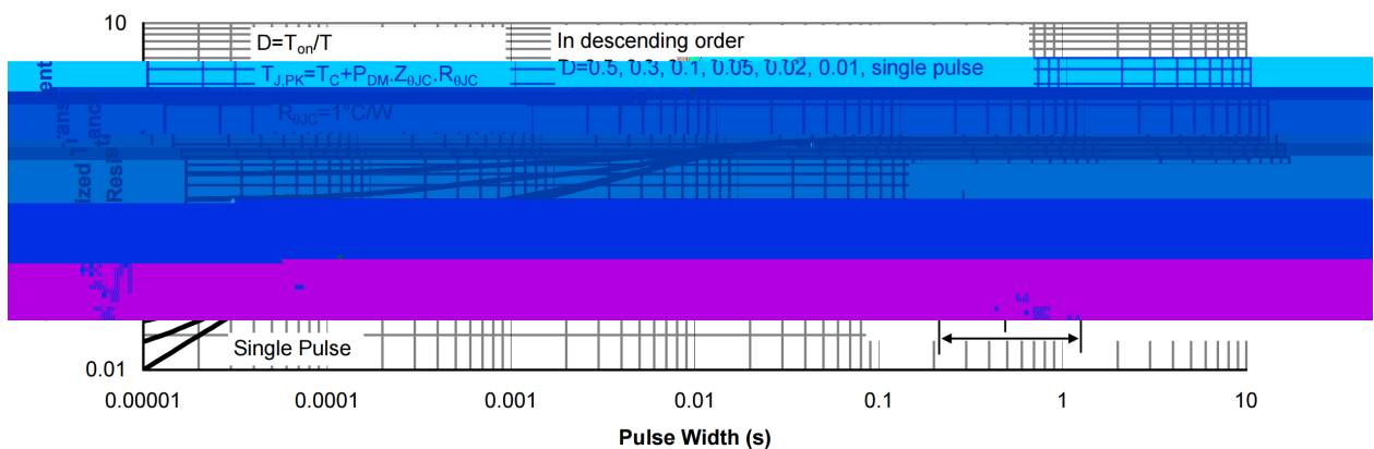
Figure 4: Normalized maximum and minimum temperatures of the pipe
