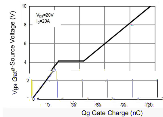
Figure 5 Gate Charge
