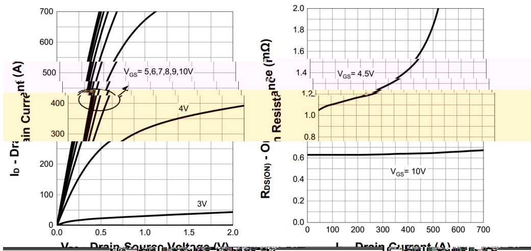
5. Output Characteristics
